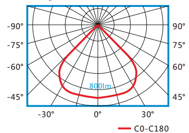
Light Distribution Curve
